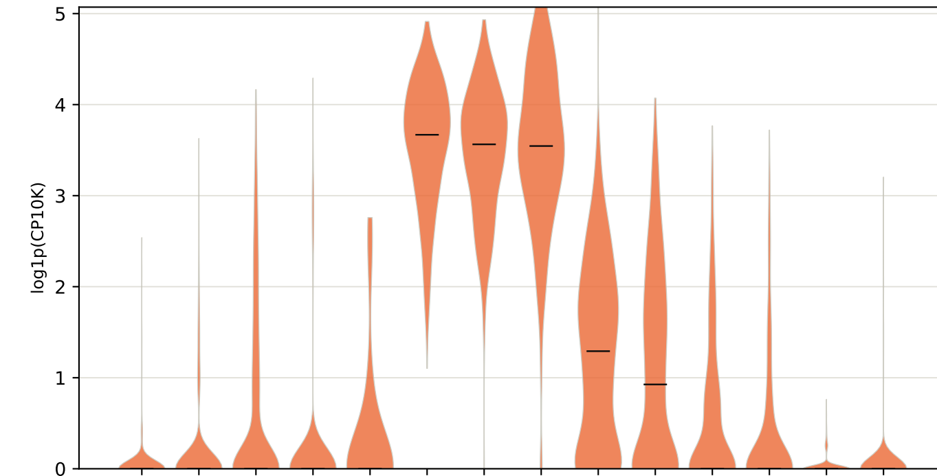
KRT17
