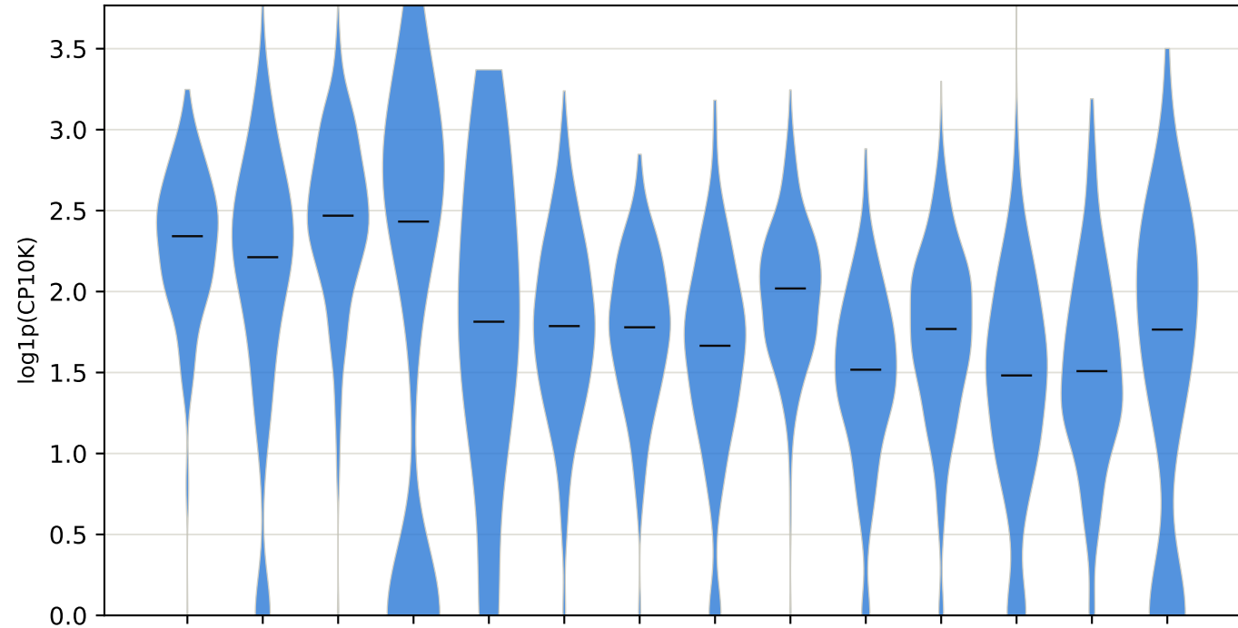
KRT8
